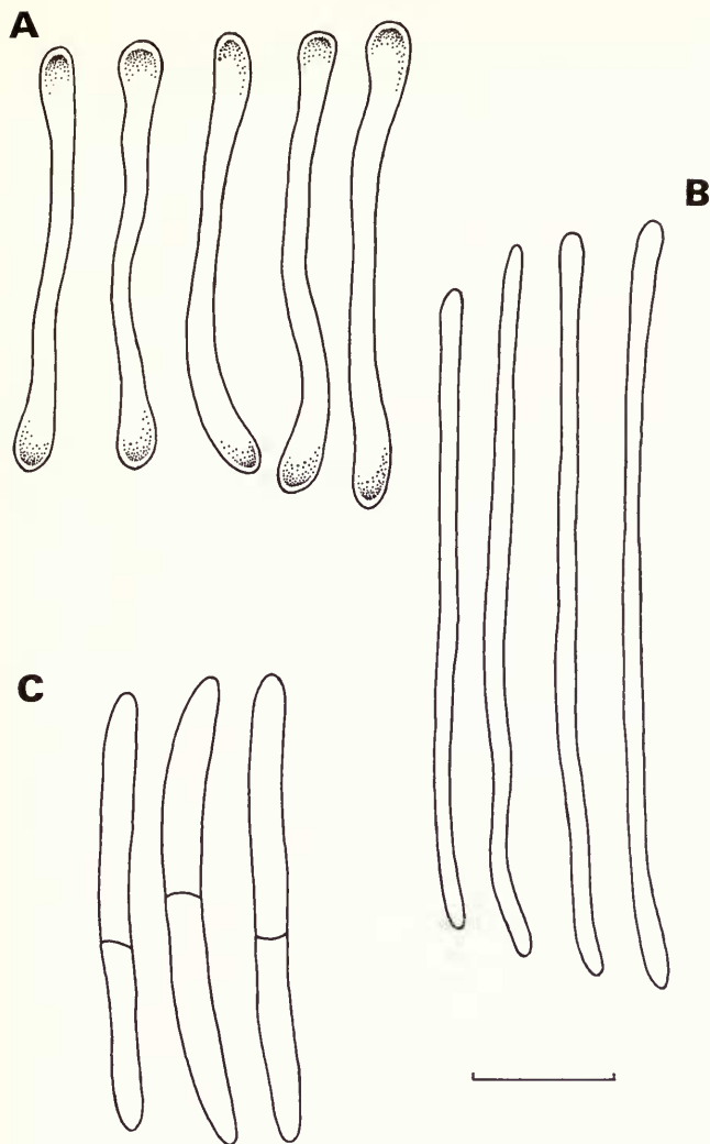
Fig. 54 Ascospore outlines (A) Sarcopyrenia gibba (Nyl.) Nyl. (H-NYL 4058-holotype); (B) Sarcopyrenia beckhausiana (Lahm) Aguirre, Nav., Ros. & Hladún (B 4488-lectotype); (C) Sarcopyrenia cylindrospora (P. Crouan & H. Crouan) Aguirre (Concarneau-holotype); scale = 10 \mu m.
